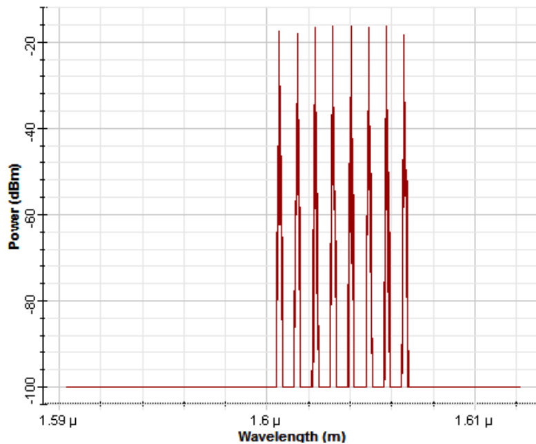
Figure 4-22: downstream wavelengths – spectrum analyzer for 40 Gbps TWDM-PON
