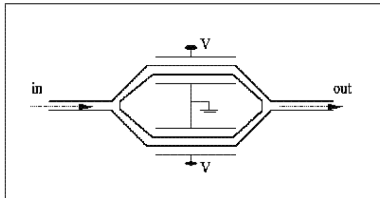
Figure 2-3: Mach-Zehnder modulator [24]
