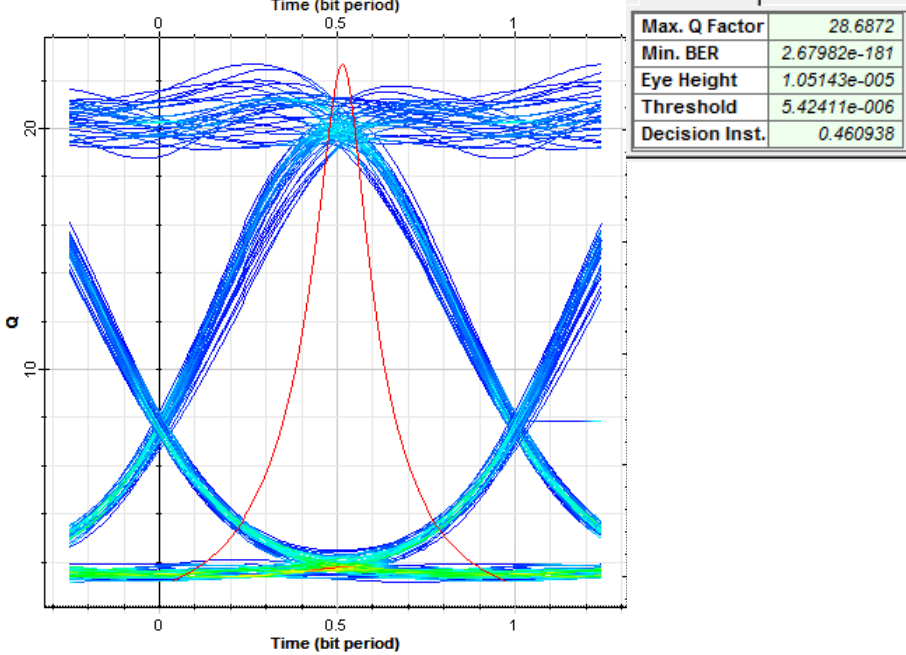
c) Eye Diagram for 1535.82 nm downstream at 40 Km
